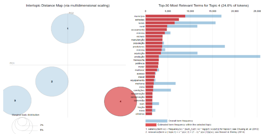
Figure 5: Multidimensional map and relevant terms of Topic 4
