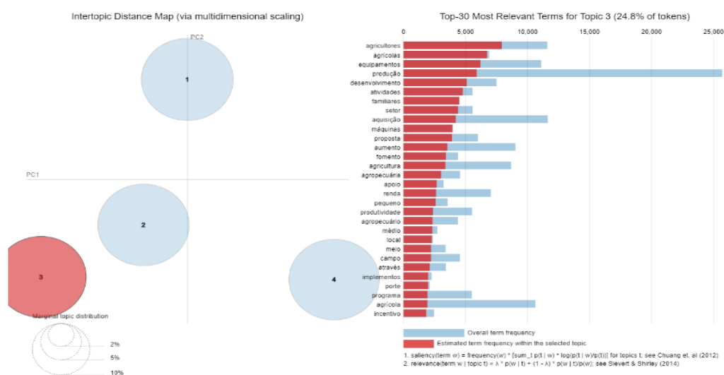
Figure 4: Multidimensional map and relevant terms of Topic 3
